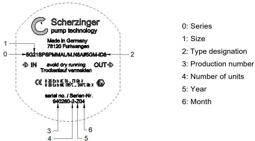
Fig. 1: Nameplate for pump with motor
