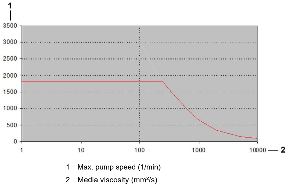
Fig. 2: Viscosity range
