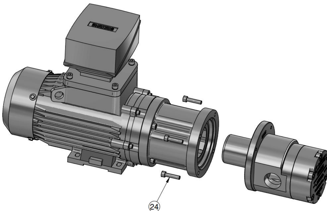
Fig. 11: Disassembly of pump head
