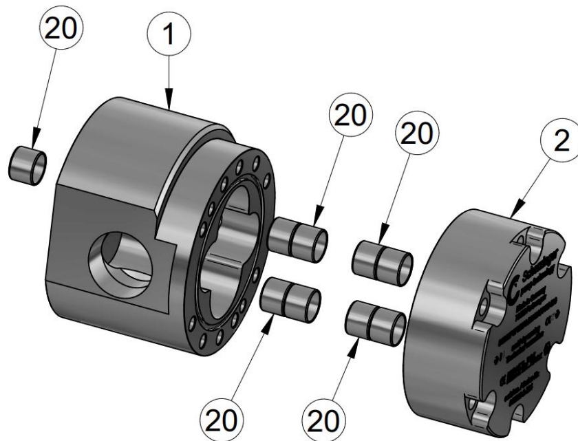
Fig. 9: Shaft bearings
