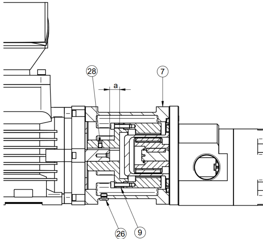
Fig. 10: Mounting the magnetic coupling
