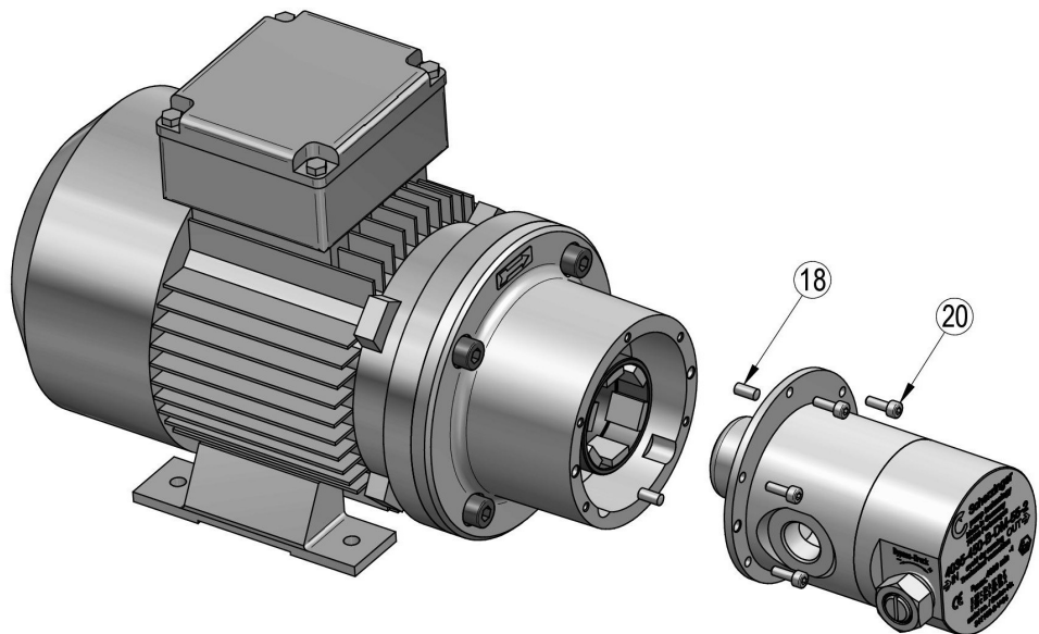
Abb. 11: Demontage Pumpenkopf
